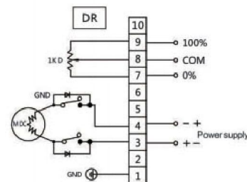
DC Circuit diagram (with potentiometer)
