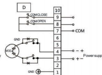
DC ON/OFF TYPE Circuit diagram
